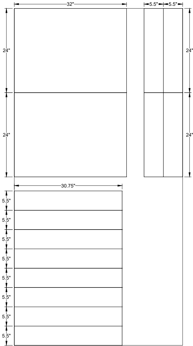
5/8" PLYWOOD
