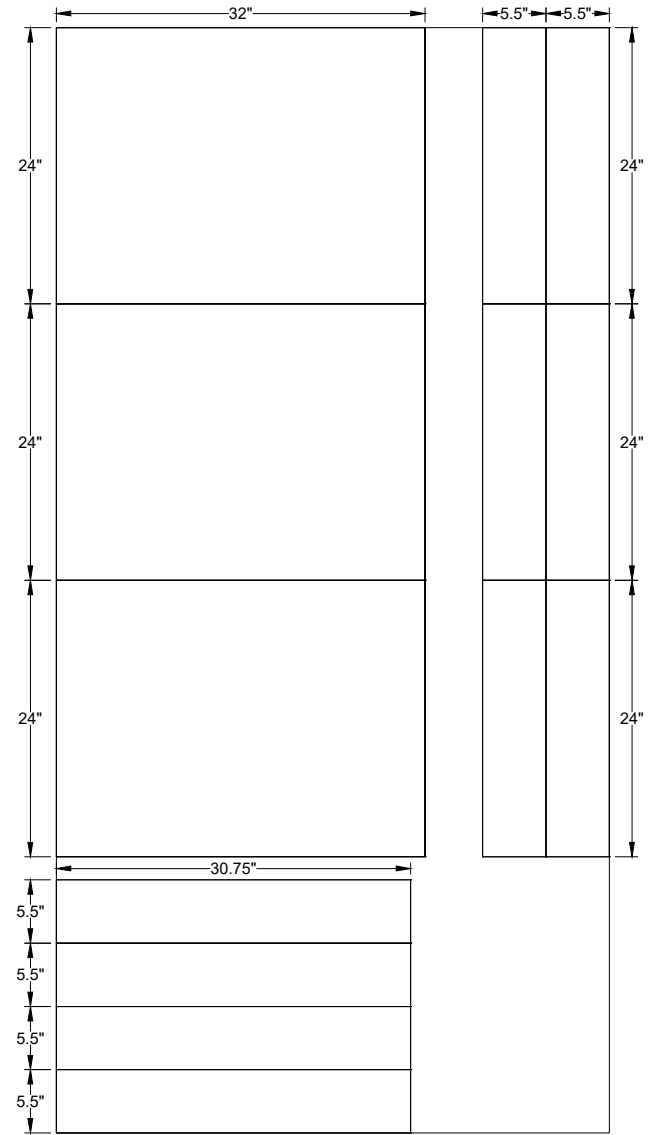
5/8" PLYWOOD
