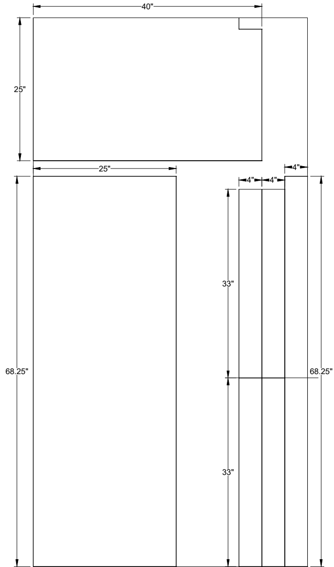
3/4" PLYWOOD
