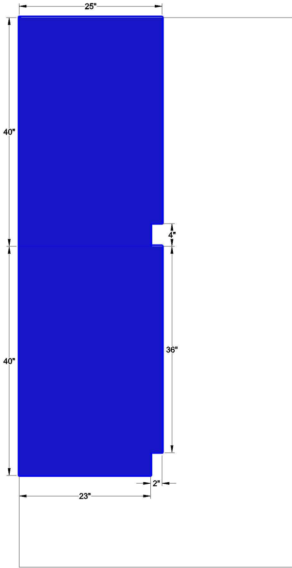
3/4" PLYWOOD
