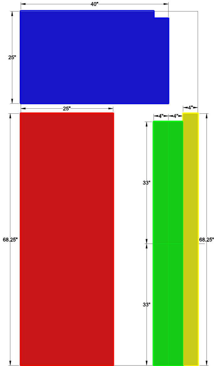
3/4" PLYWOOD
